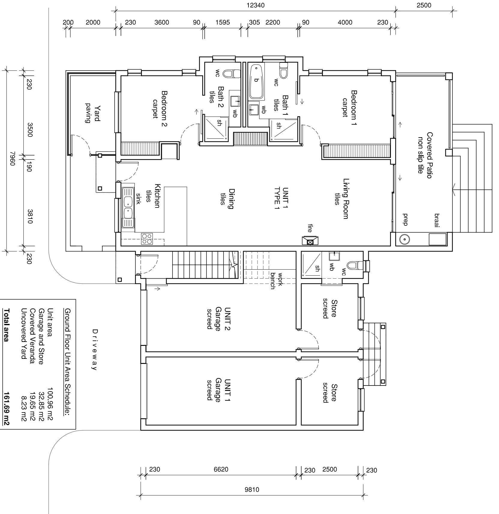
TYPICAL 2 BEDROOM 2 BATHROOM UNIT GROUND FLOOR PLAN
