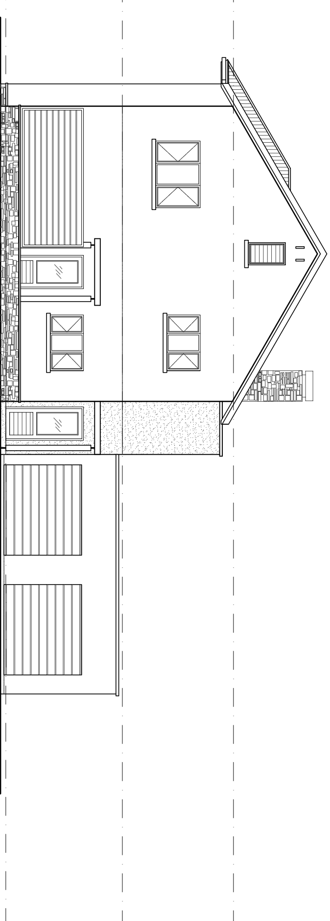
TYPICAL 2 BEDROOM 2 BATHROOM UNIT REAR ENTRANCE ELEVATION
